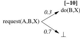
Figure 1: A frame repository based on the SRP, compiled into a tree.
